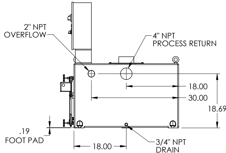
BACK VIEW
